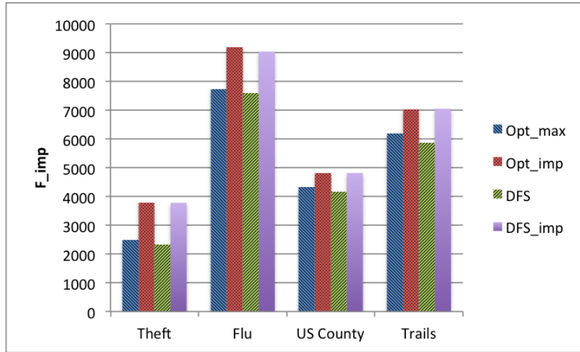
Fig. 8. Objective Based on Importance with Zipfian Distribution
