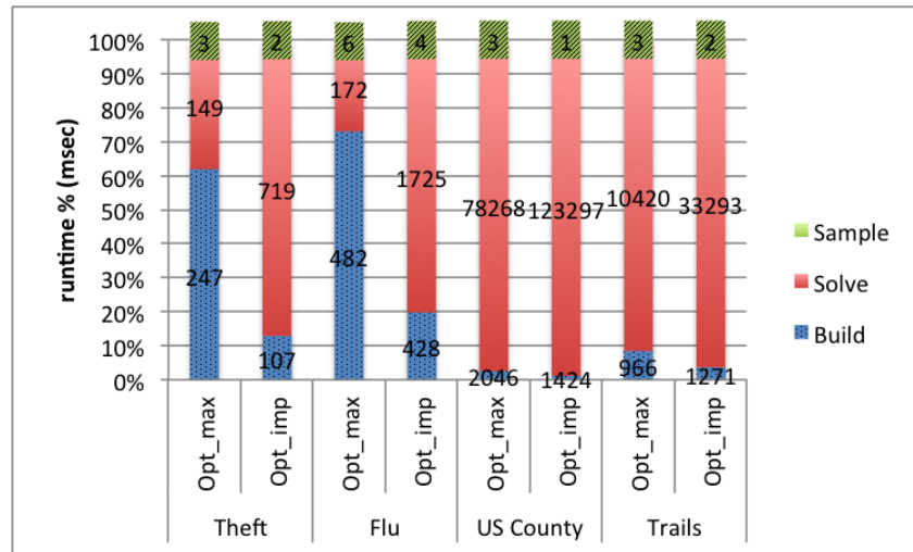
Fig. 10. Breakup of Runtime
