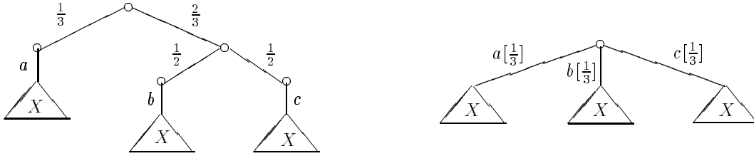
Figure 2: Stratified and generative transition systems of Sc' .
