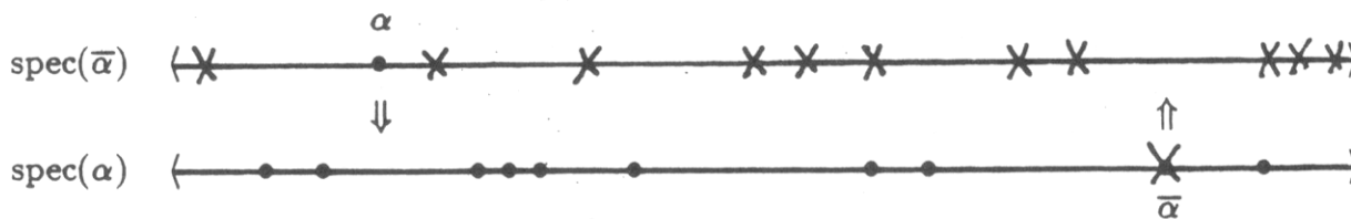
Figure B. By hypothesis, either \alpha \in \text{spec}(\bar{\alpha}) , or \bar{\alpha} \in \text{spec}(\alpha) . Here \alpha is not in \text{spec}(\bar{\alpha}) , so \bar{\alpha} must be \text{spec}(\alpha) .
